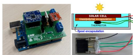
Figure 5: The Perovskino MPP tracker driving a high hysteresis perovskite solar cell[4].
